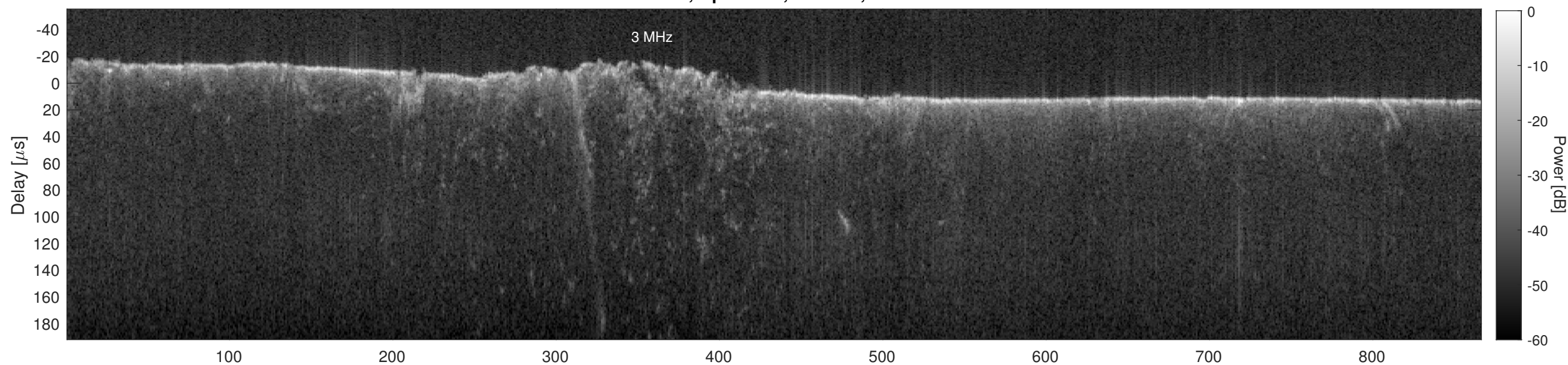
Orbit 14222, Cluttergram
