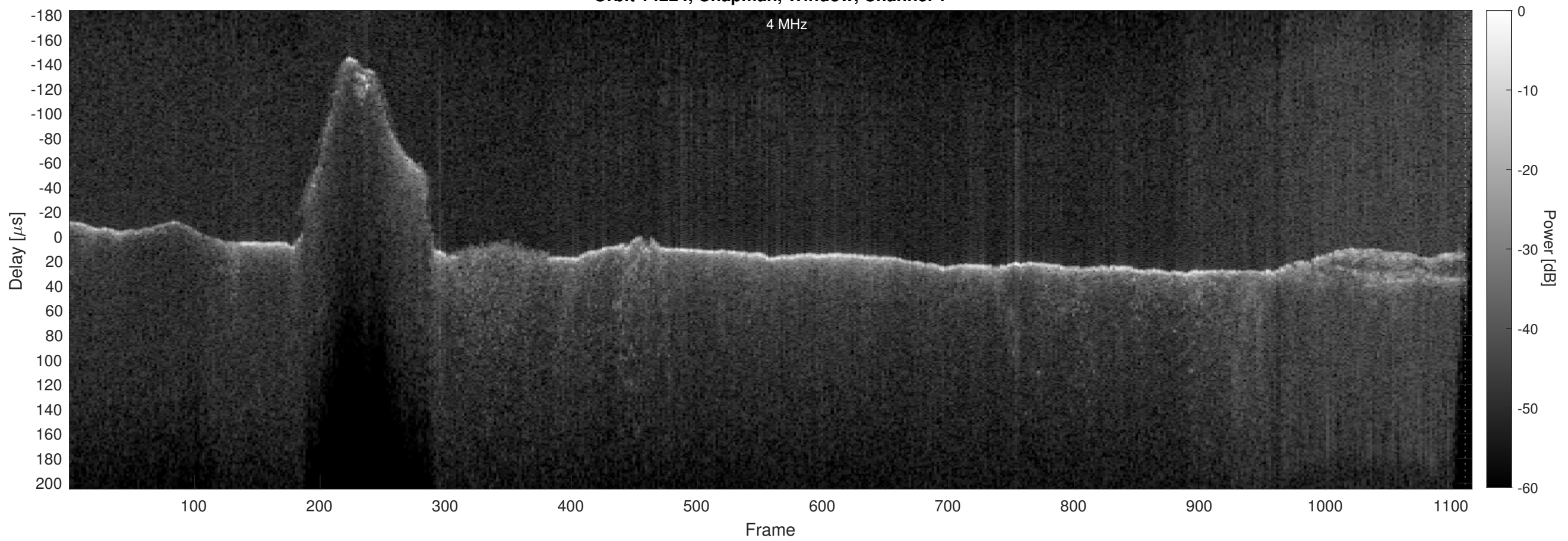
Orbit 14224, Chapman, Window, Channel 2
