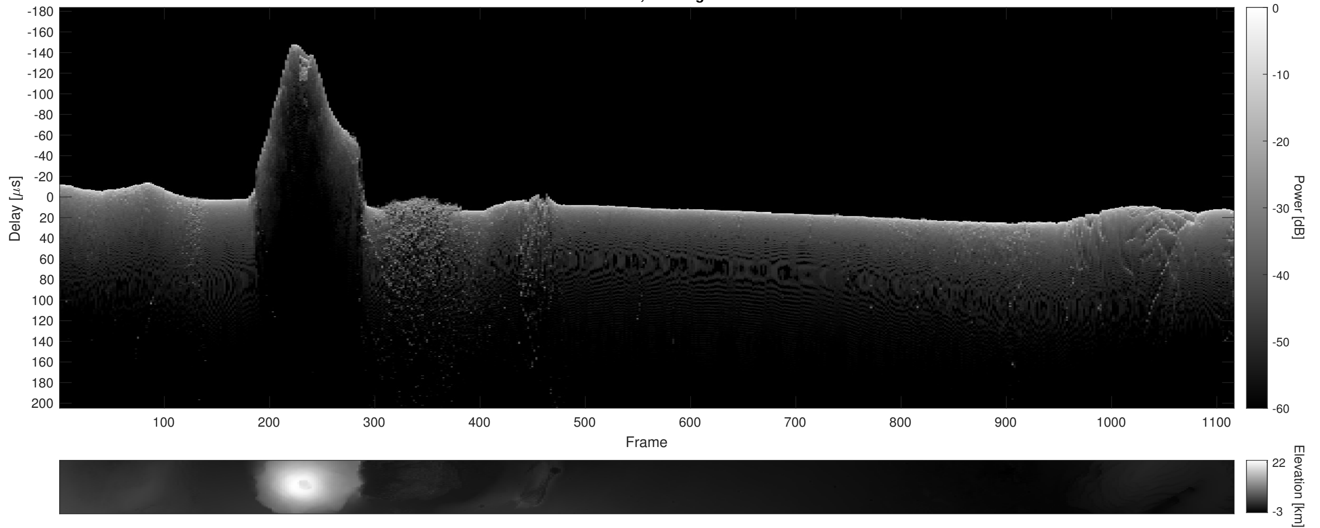
Orbit 14224, Cluttergram
