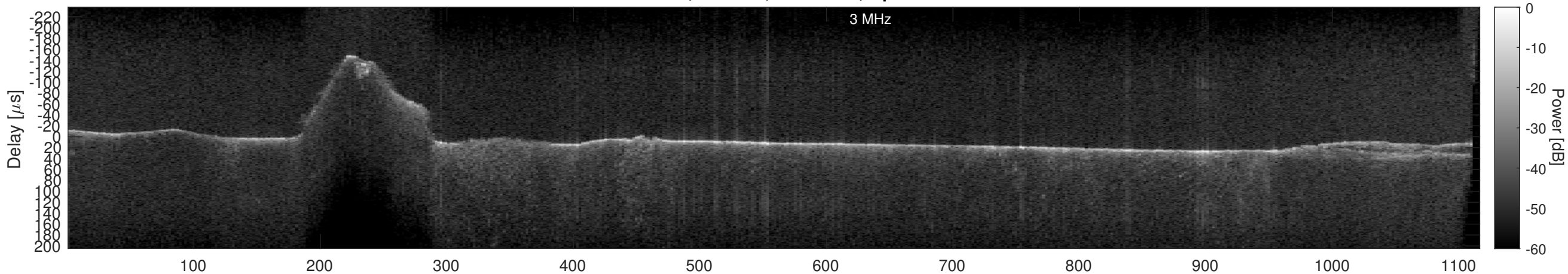
Orbit 14224, Cluttergram
