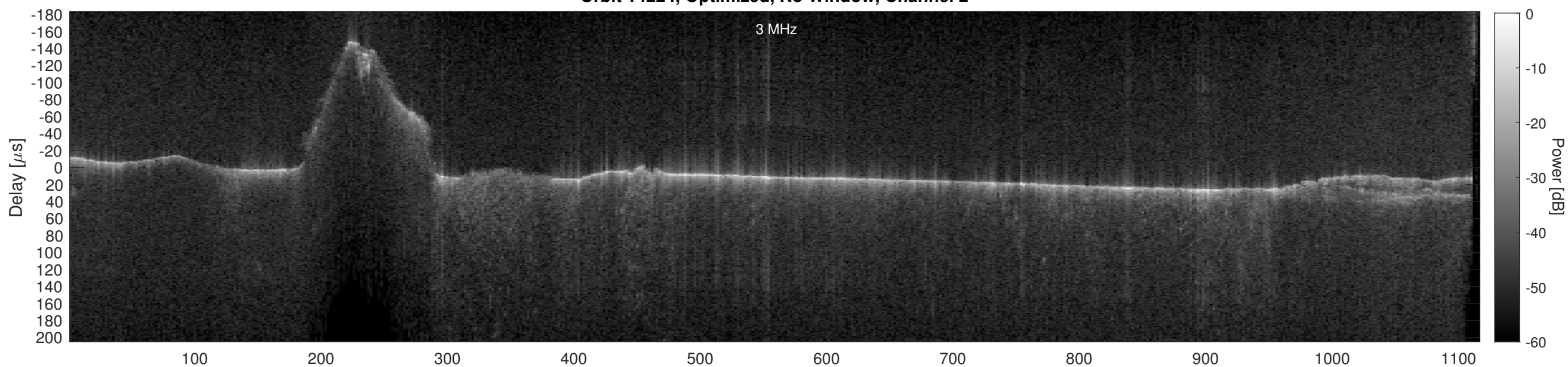
Orbit 14224, Cluttergram
