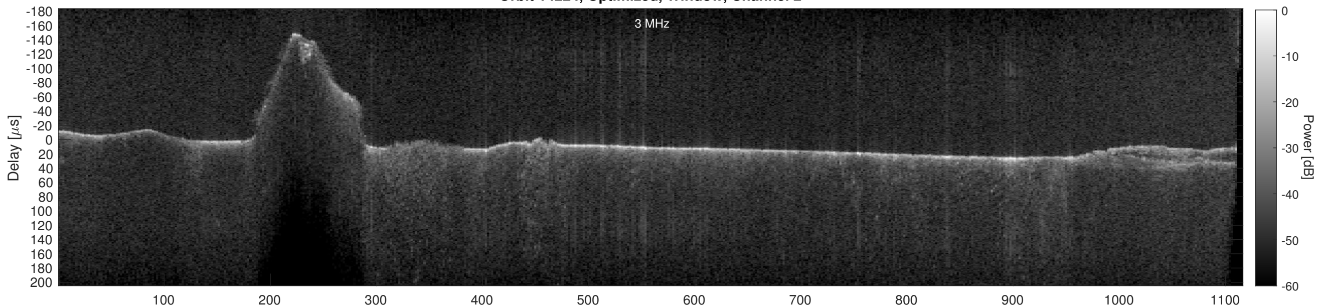
Orbit 14224, Cluttergram
