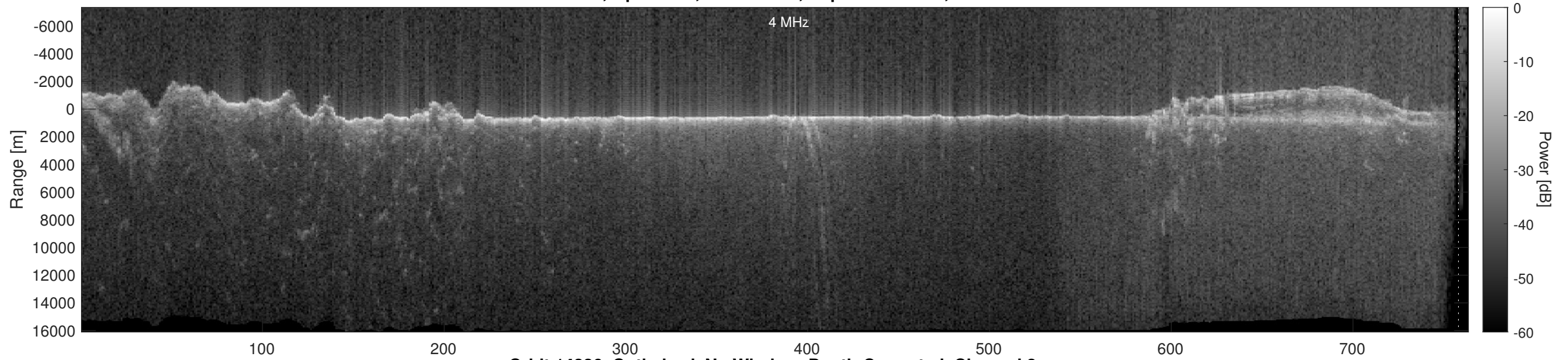
Orbit 14226, Optimized, No Window, Depth-Corrected, Channel 2
