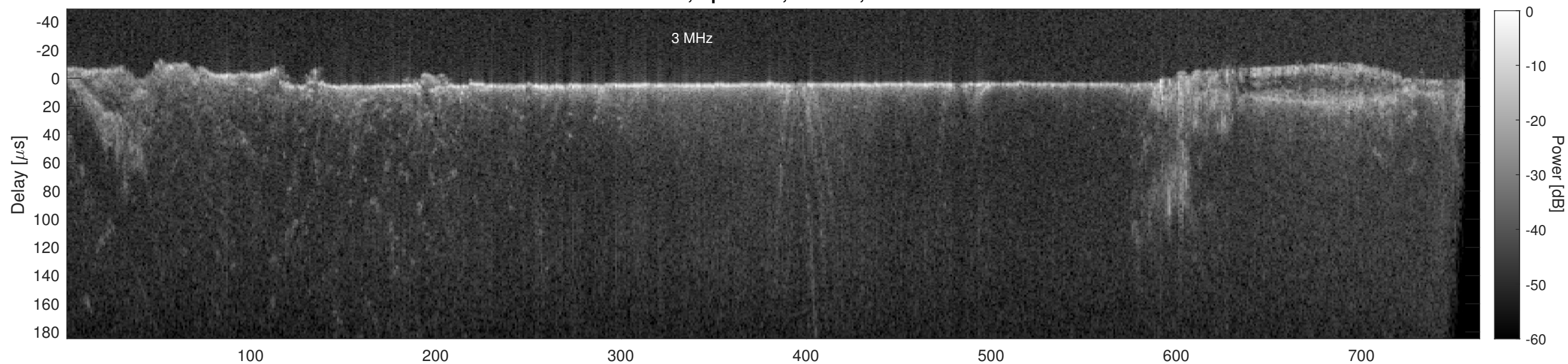
Orbit 14226, Cluttergram
