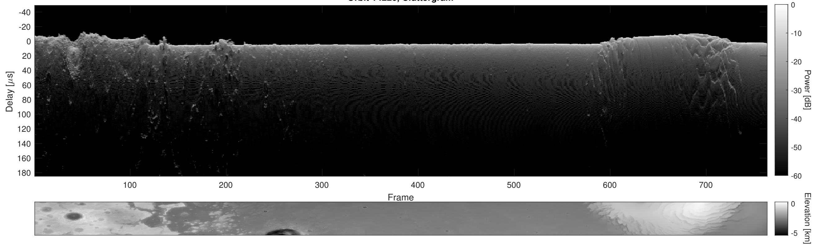
Orbit 14226, Cluttergram
