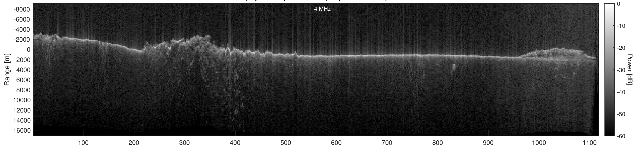
Orbit 14229, Optimized, No Window, Depth-Corrected, Channel 2
