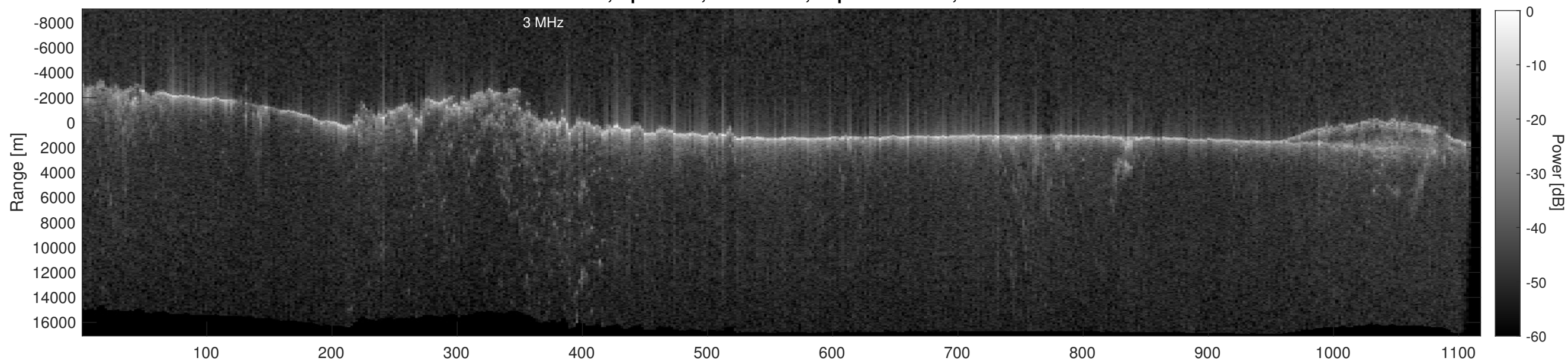
Orbit 14229, Depth-Corrected Cluttergram
