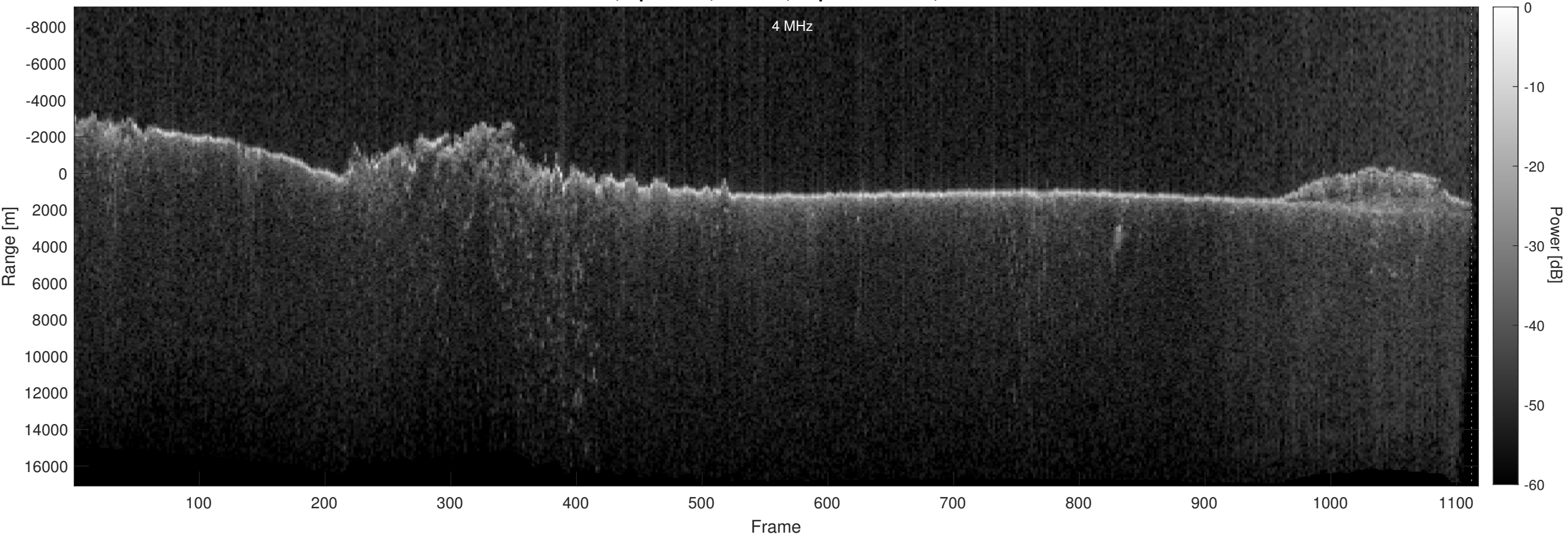
Orbit 14229, Optimized, Window, Depth-Corrected, Channel 2
