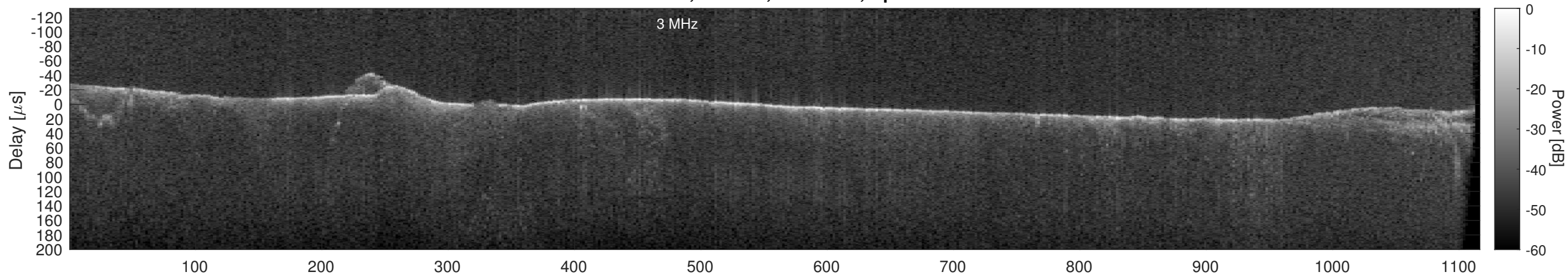
Orbit 14231, Cluttergram
