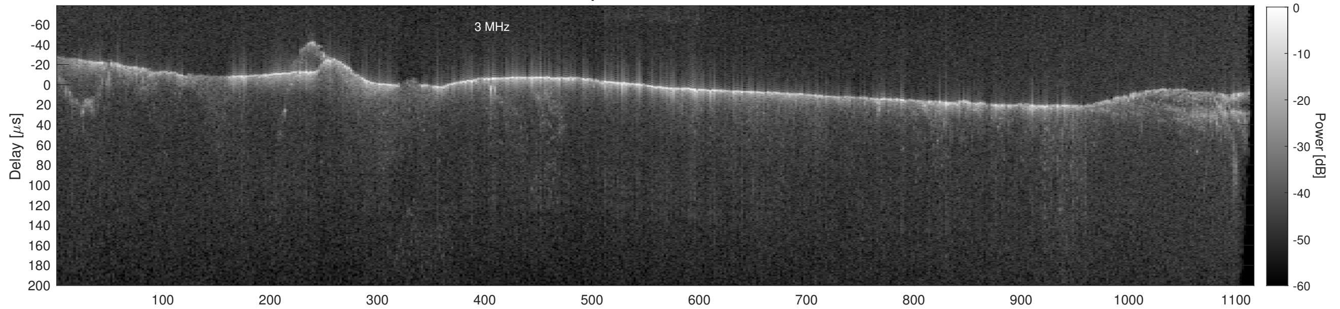
Orbit 14231, Cluttergram
