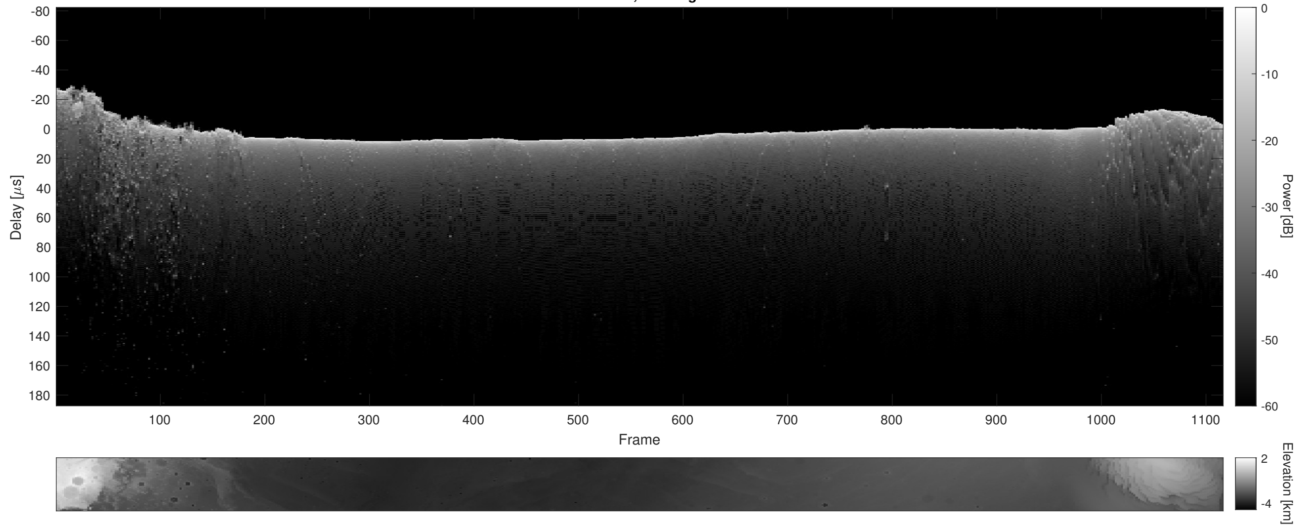
Orbit 14232, Cluttergram
