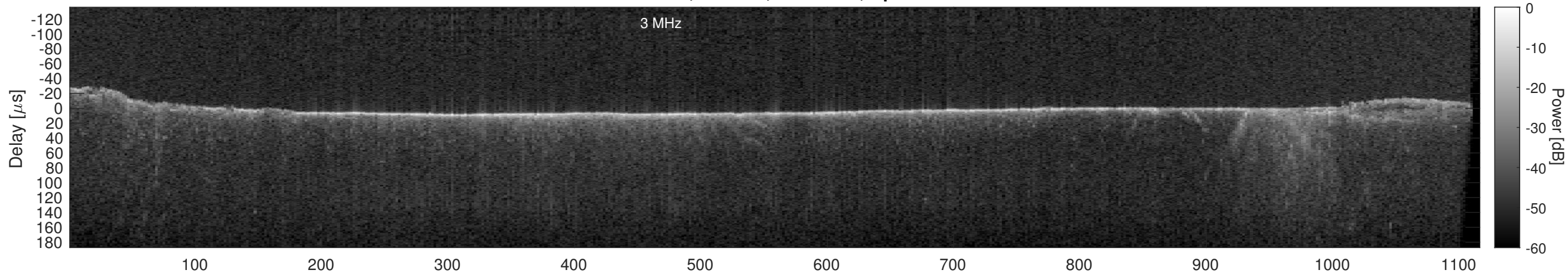
Orbit 14232, Cluttergram
