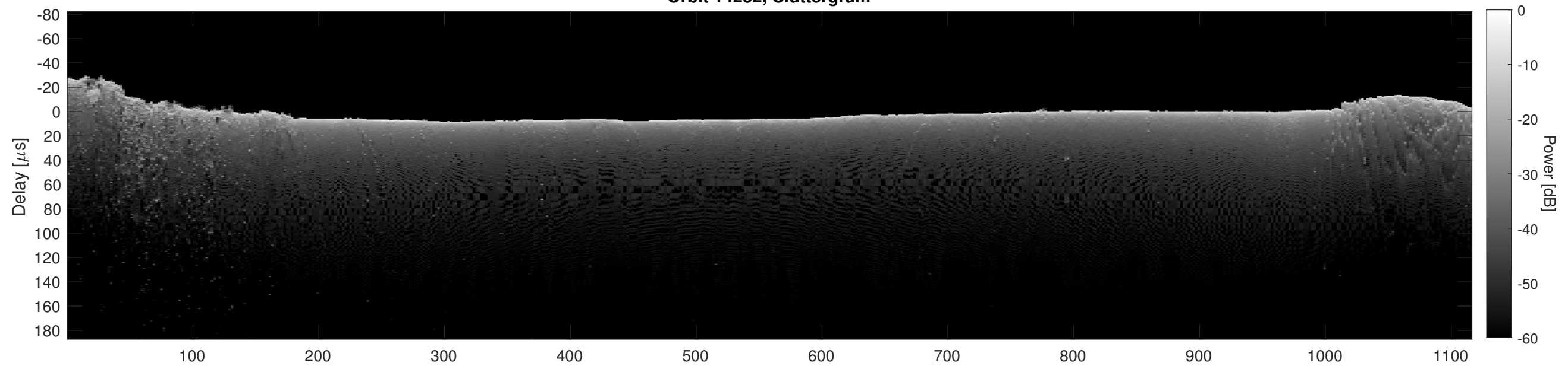
Orbit 14232, Cluttergram
