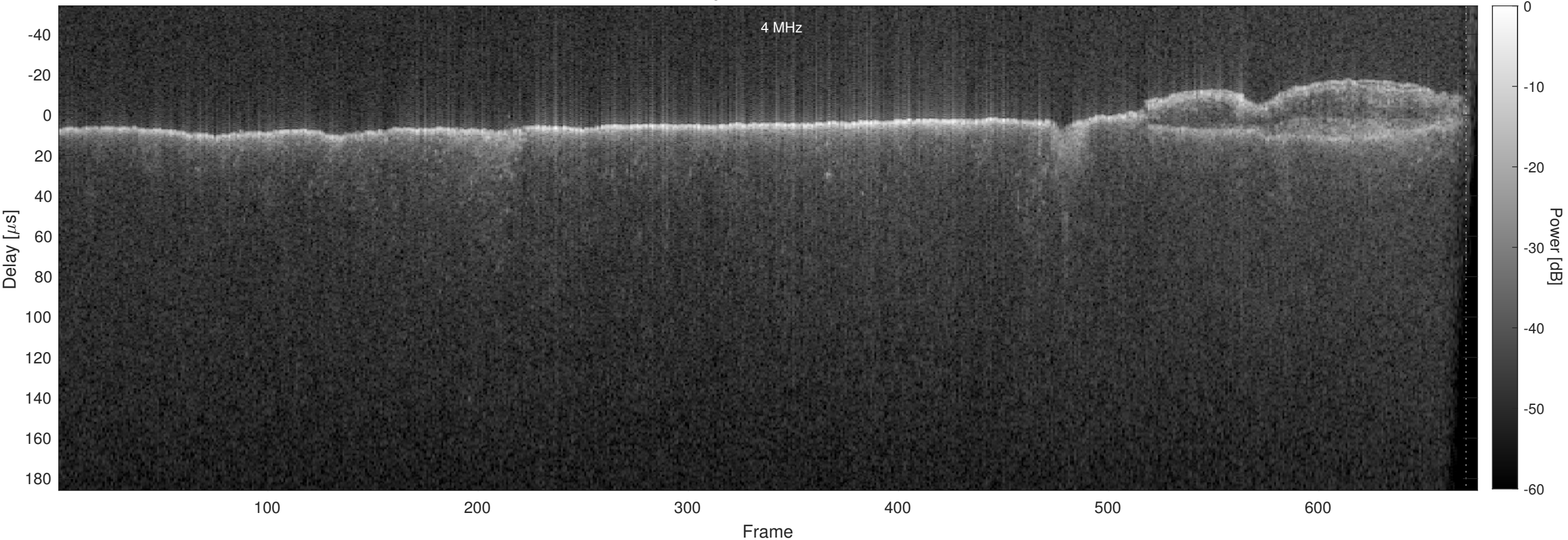
Orbit 14237, Chapman, No Window, Channel 2
