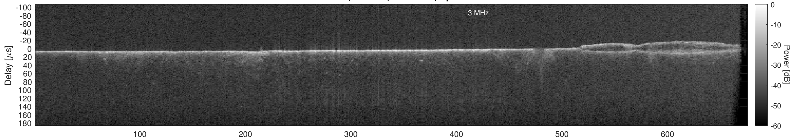
Orbit 14237, Cluttergram
