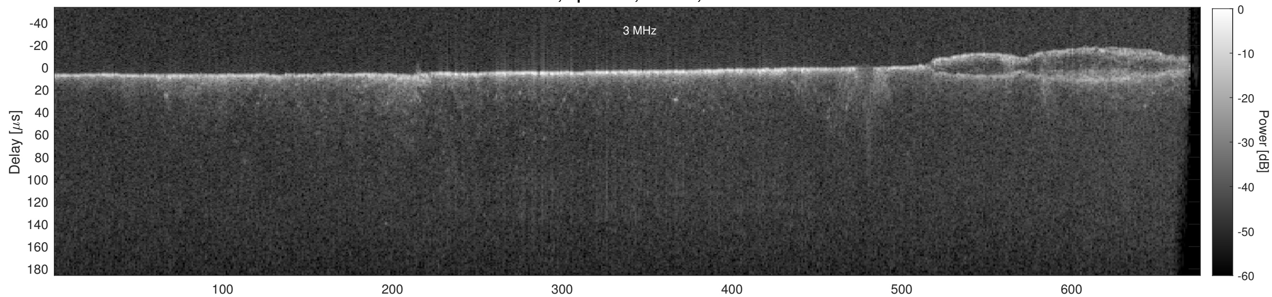
Orbit 14237, Cluttergram
