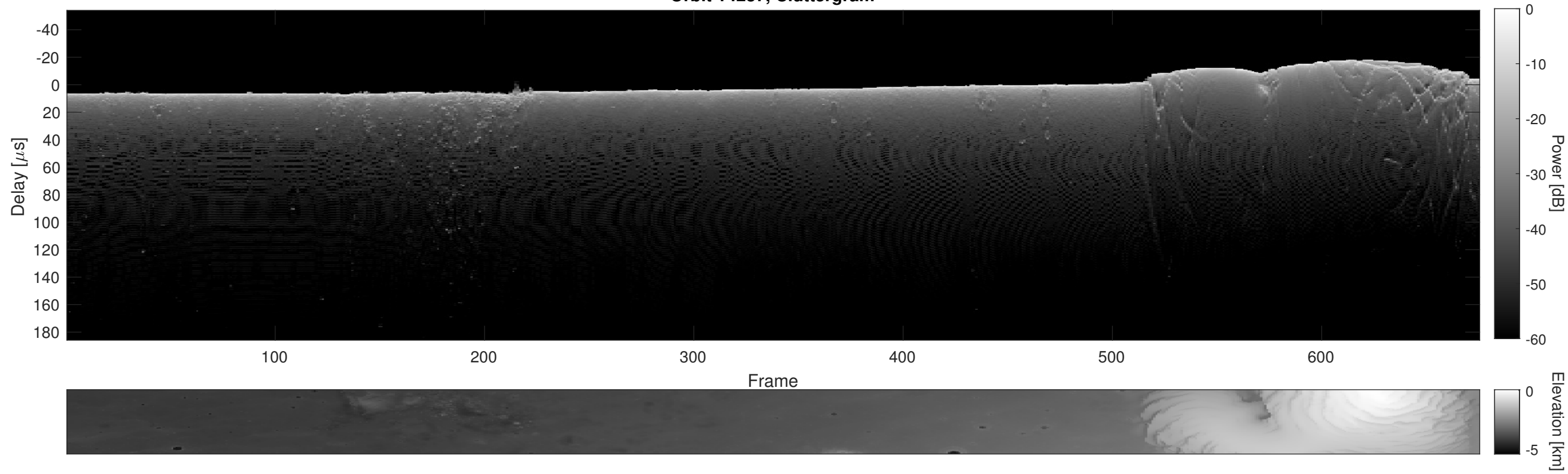
Orbit 14237, Cluttergram
