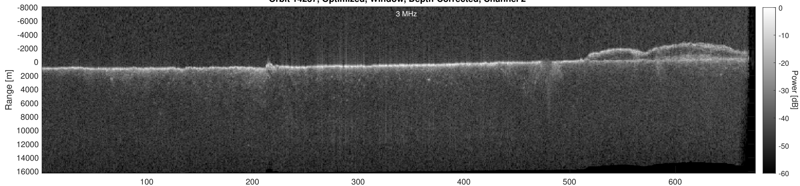
Orbit 14237, Depth-Corrected Cluttergram
