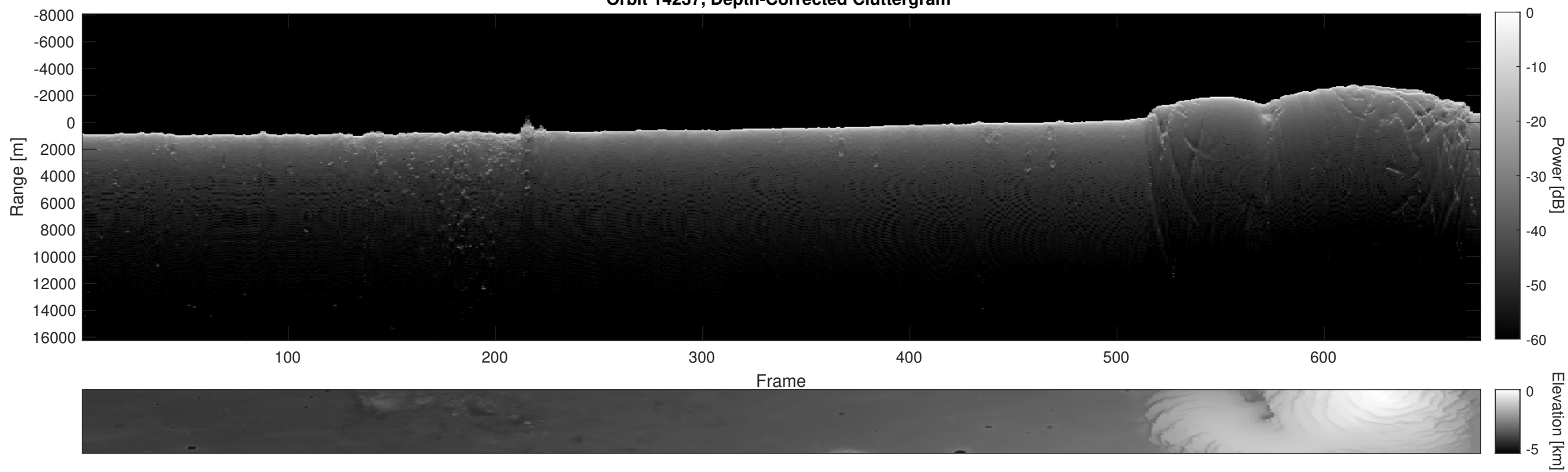
Orbit 14237, Depth-Corrected Cluttergram
