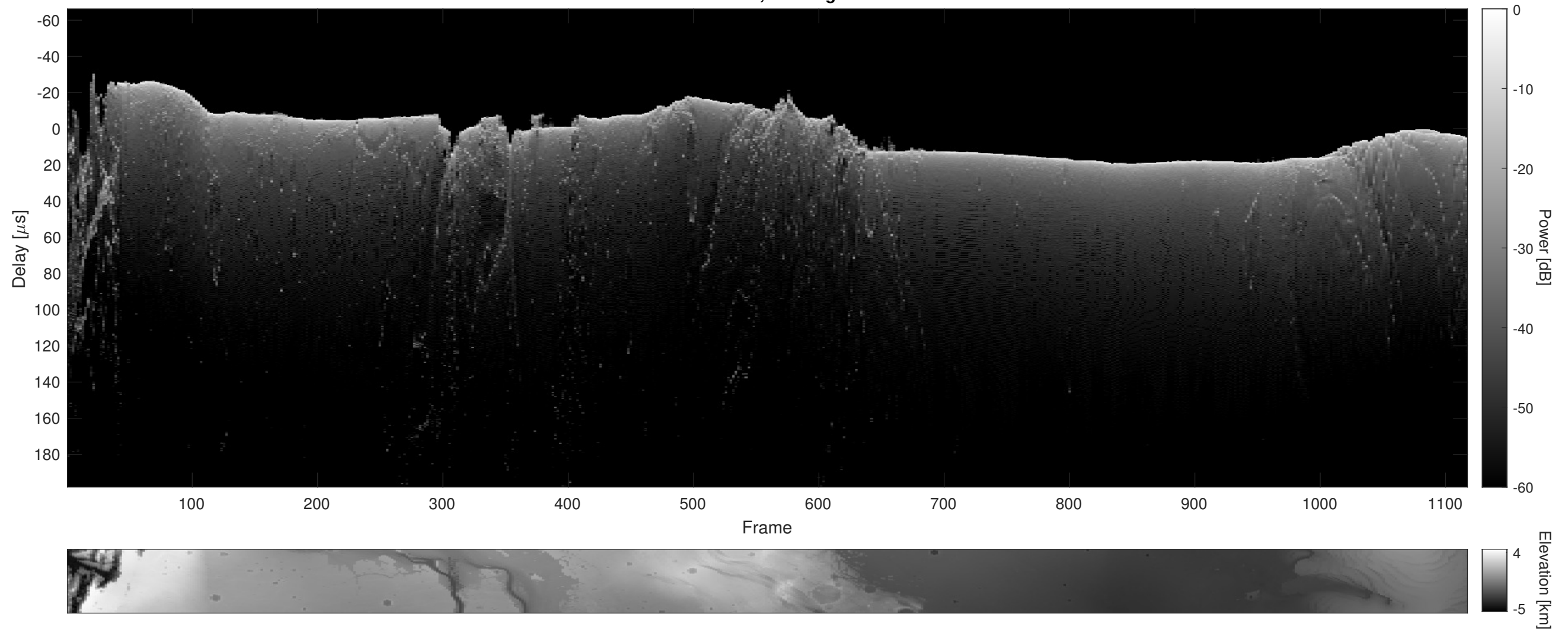
Orbit 14241, Cluttergram
