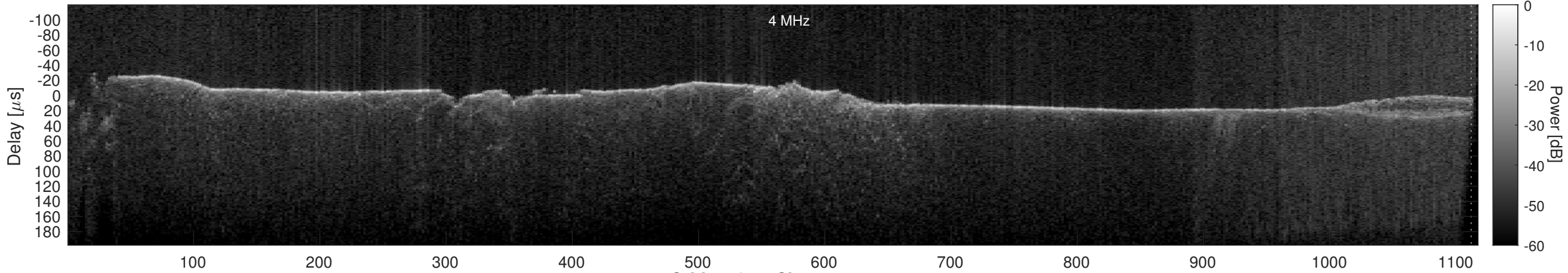
Orbit 14241, Cluttergram
