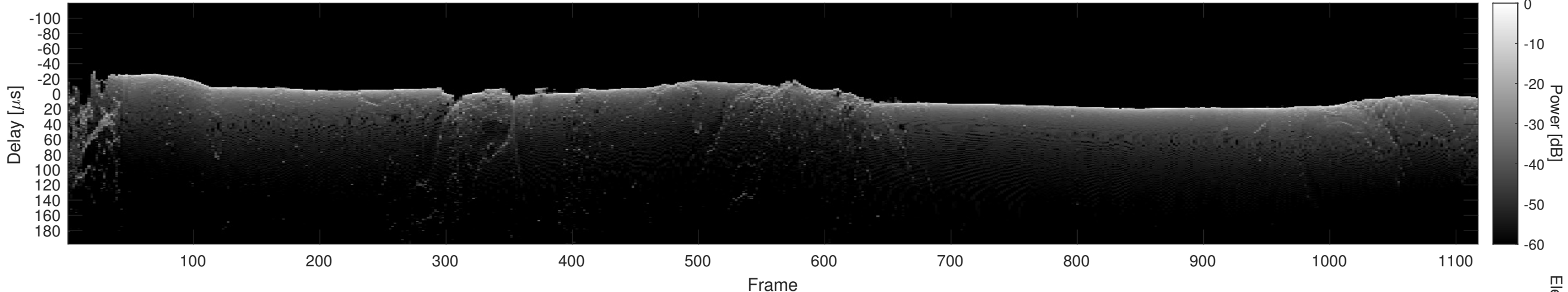
Orbit 14241, Cluttergram
