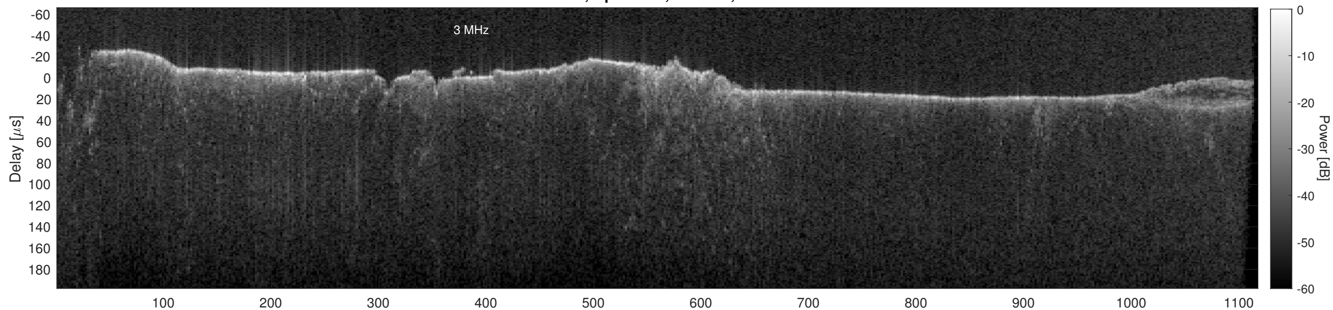
Orbit 14241, Cluttergram
