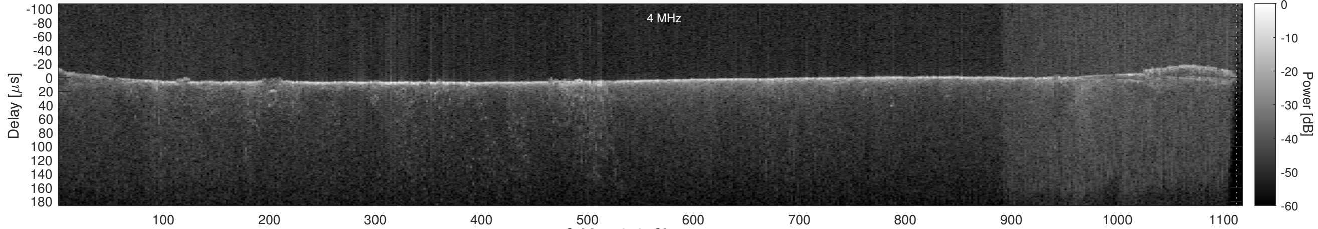
Orbit 14242, Cluttergram
