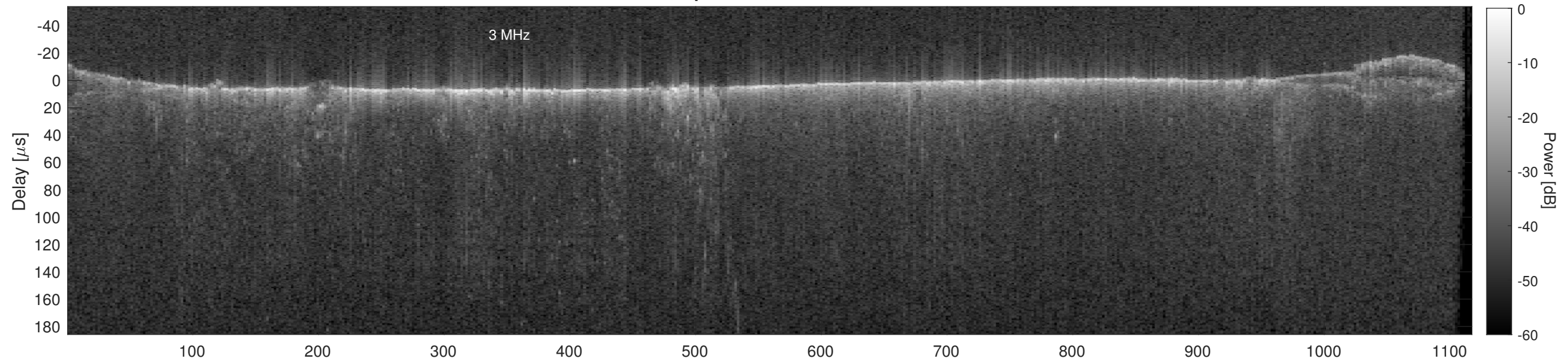
Orbit 14242, Cluttergram
