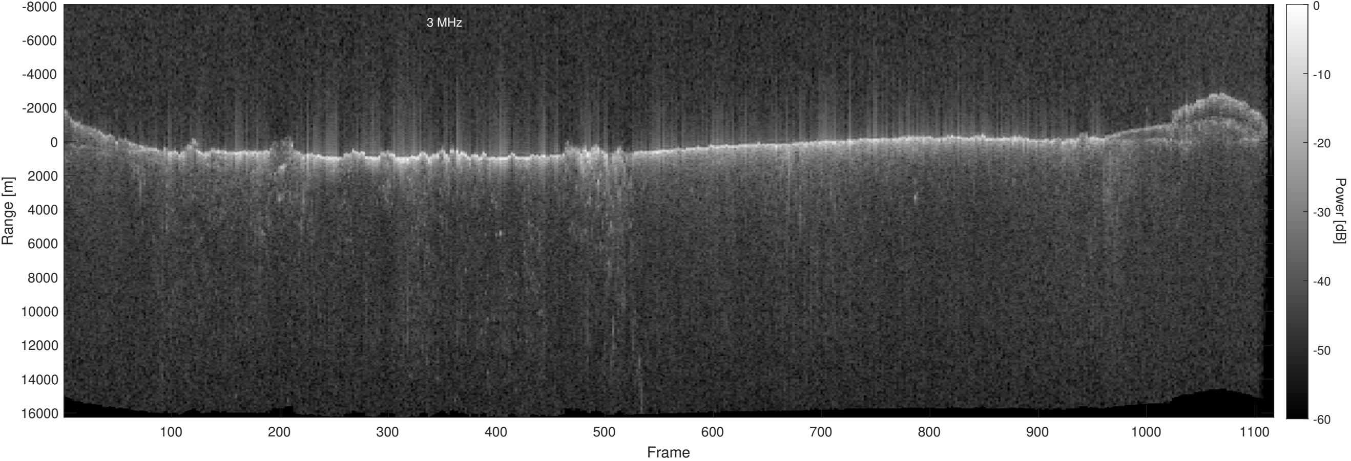
Orbit 14242, Optimized, No Window, Depth-Corrected, Channel 2
