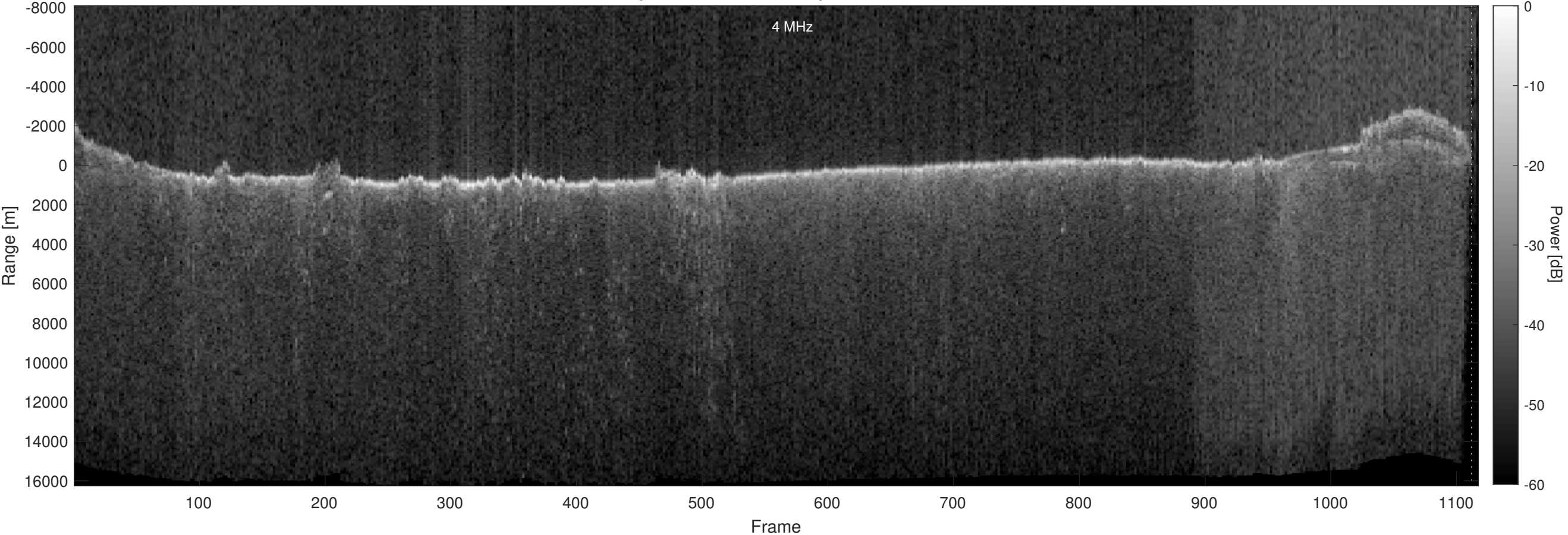
Orbit 14242, Optimized, Window, Depth-Corrected, Channel 2
