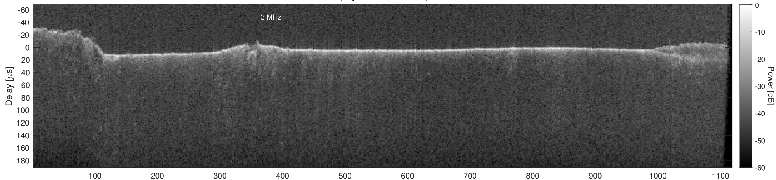
Orbit 14243, Cluttergram
