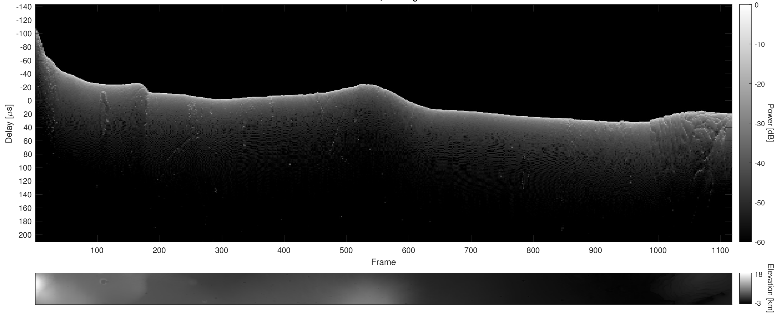
Orbit 14245, Cluttergram
