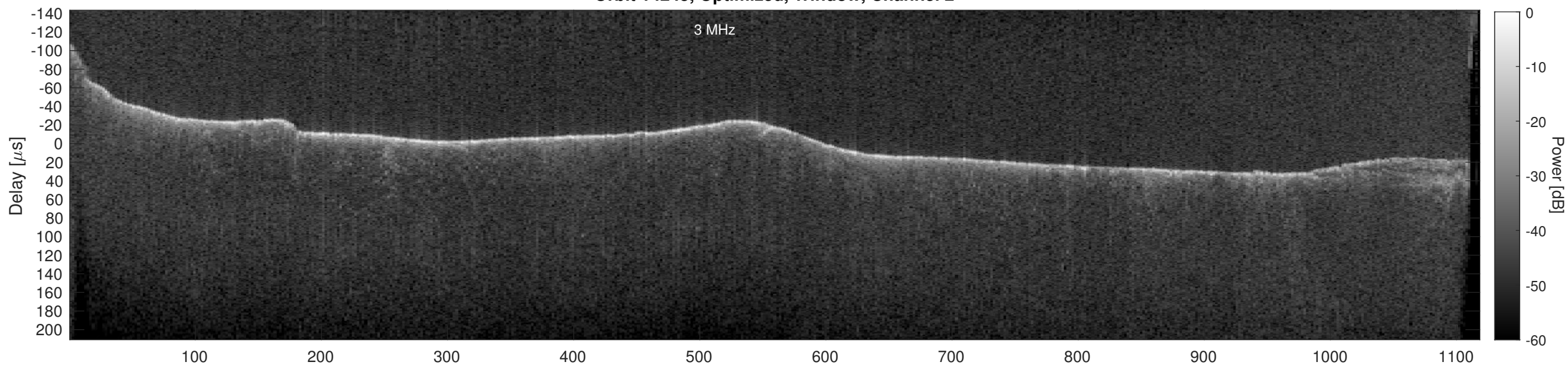
Orbit 14245, Cluttergram
