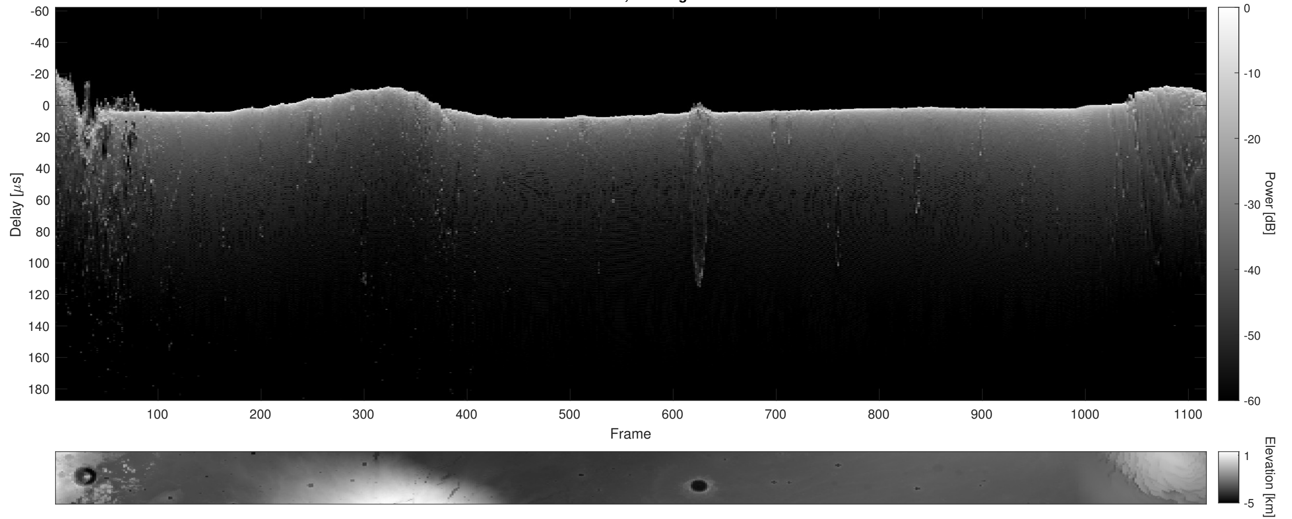
Orbit 14246, Cluttergram
