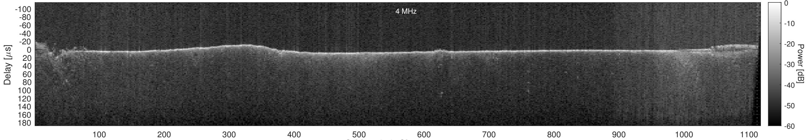
Orbit 14246, Cluttergram
