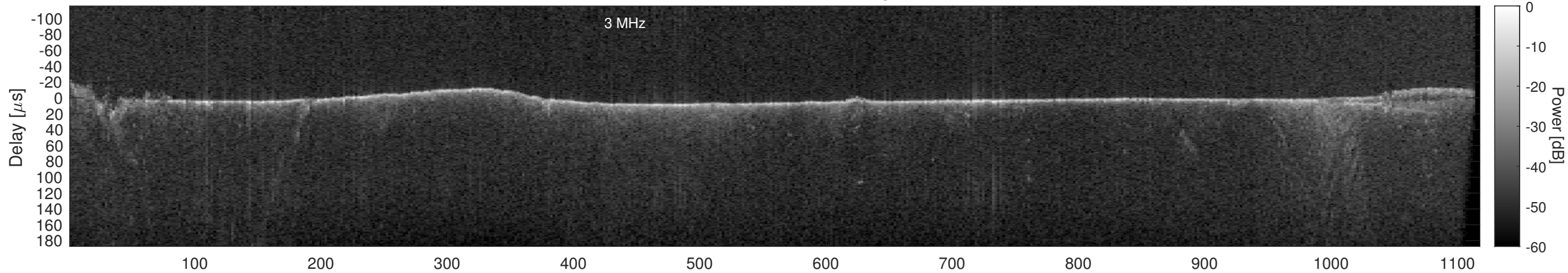
Orbit 14246, Cluttergram
