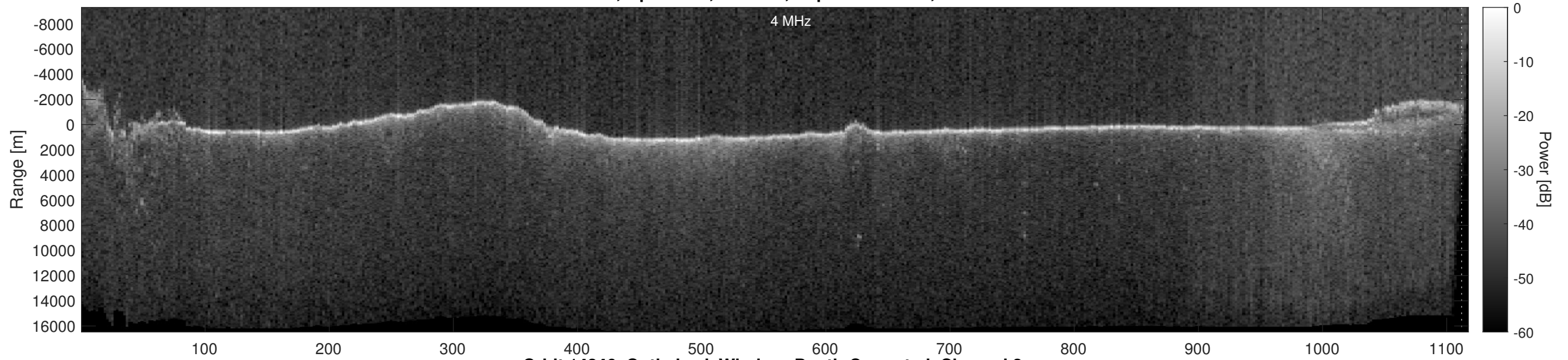
Orbit 14246, Optimized, Window, Depth-Corrected, Channel 2
