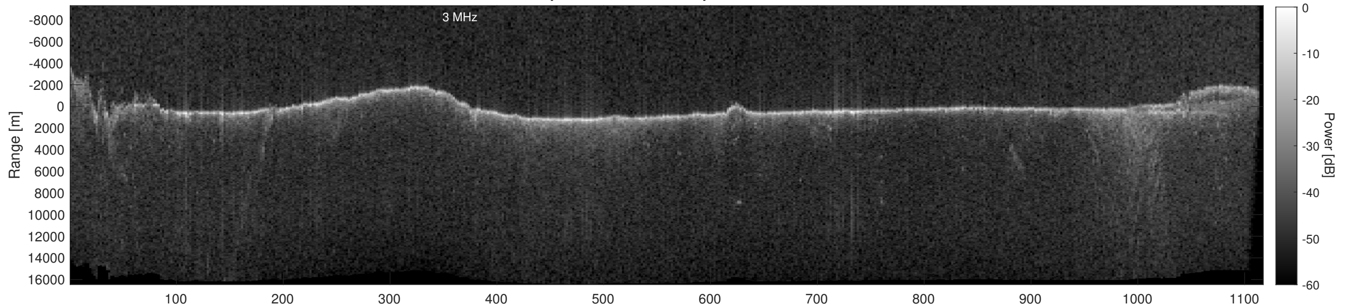
Orbit 14246, Depth-Corrected Cluttergram
