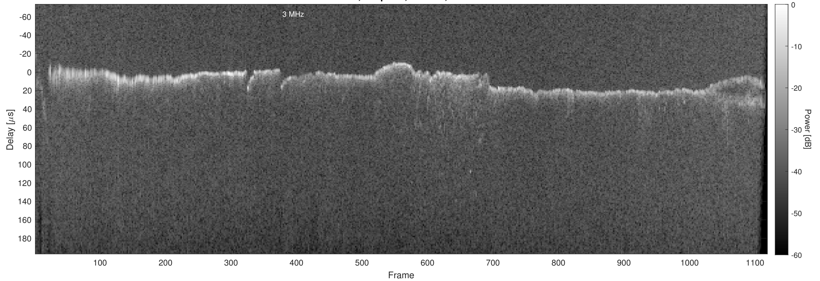
Orbit 14248, Chapman, Window, Channel 2
