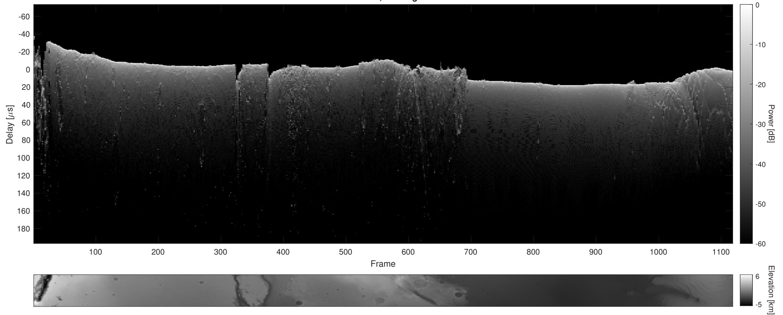
Orbit 14248, Cluttergram
