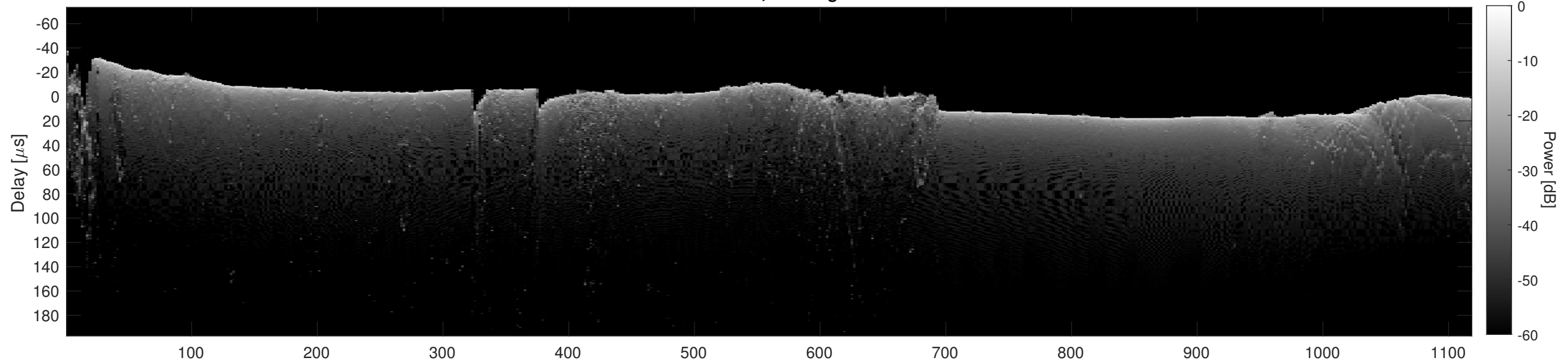
Orbit 14248, Cluttergram
