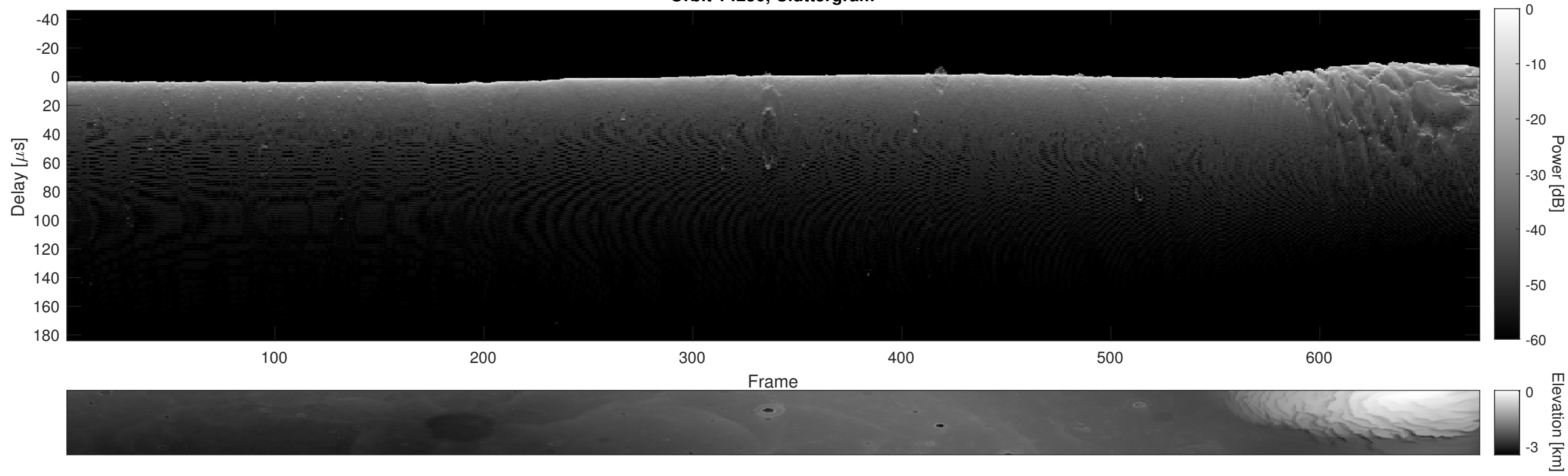
Orbit 14250, Cluttergram
