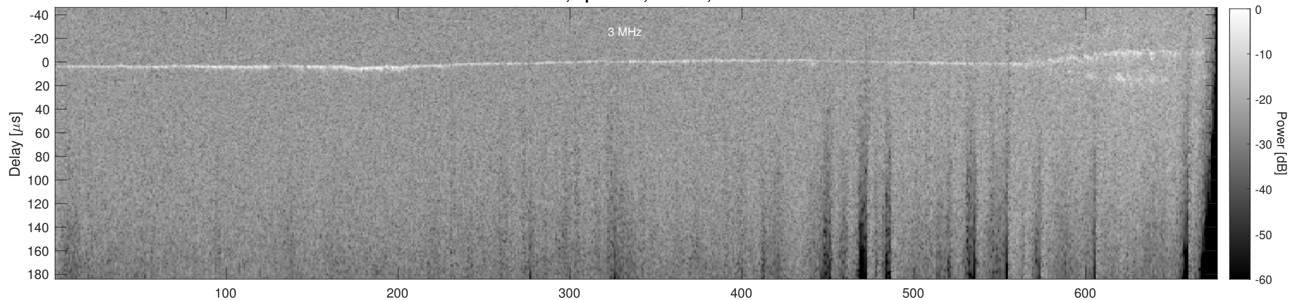
Orbit 14250, Cluttergram
