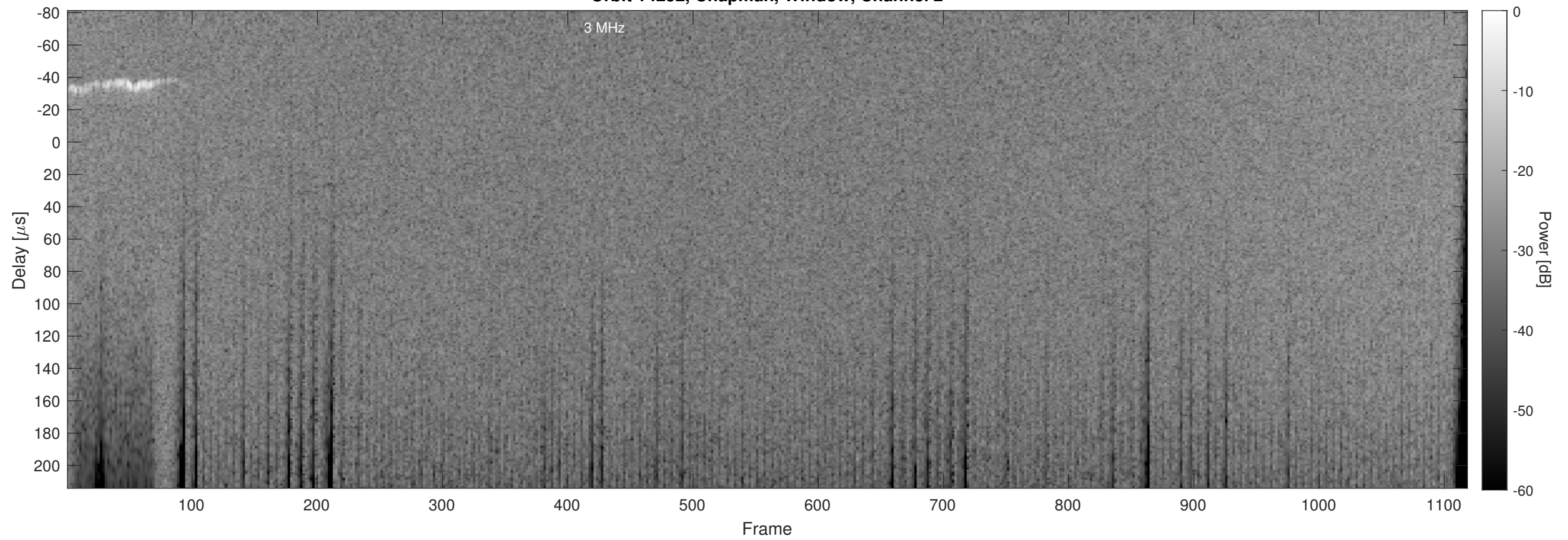
Orbit 14252, Chapman, Window, Channel 2
