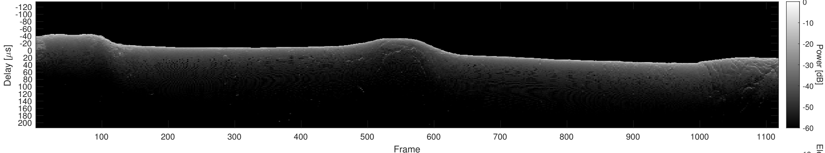
Orbit 14252, Cluttergram
