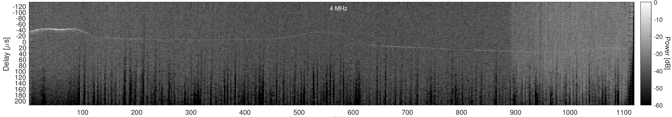
Orbit 14252, Cluttergram
