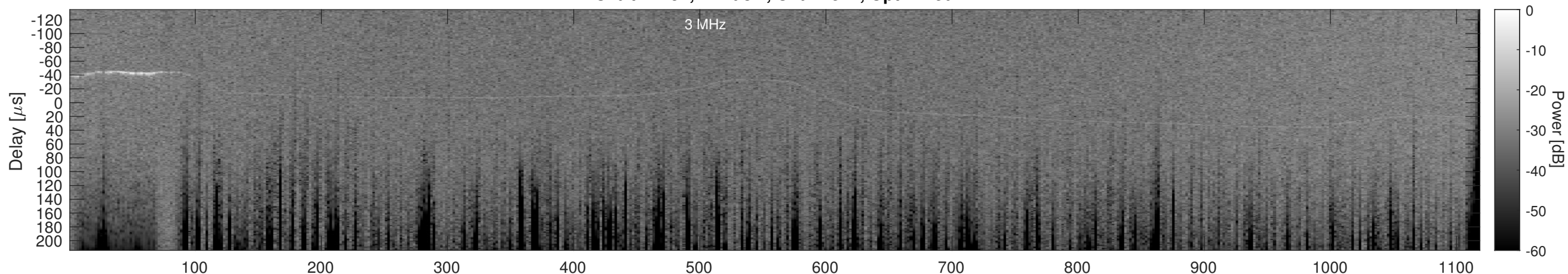
Orbit 14252, Cluttergram
