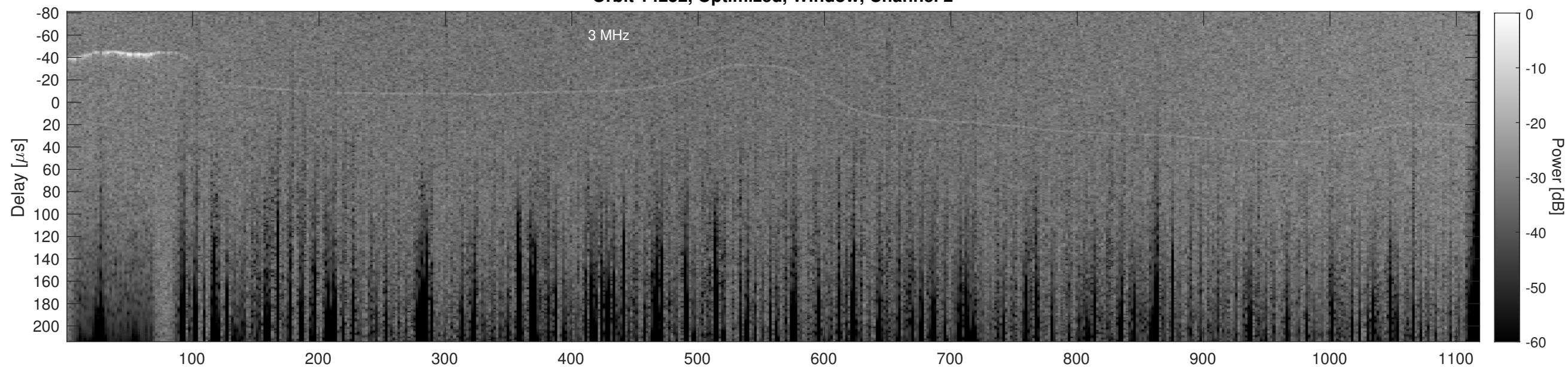
Orbit 14252, Cluttergram
