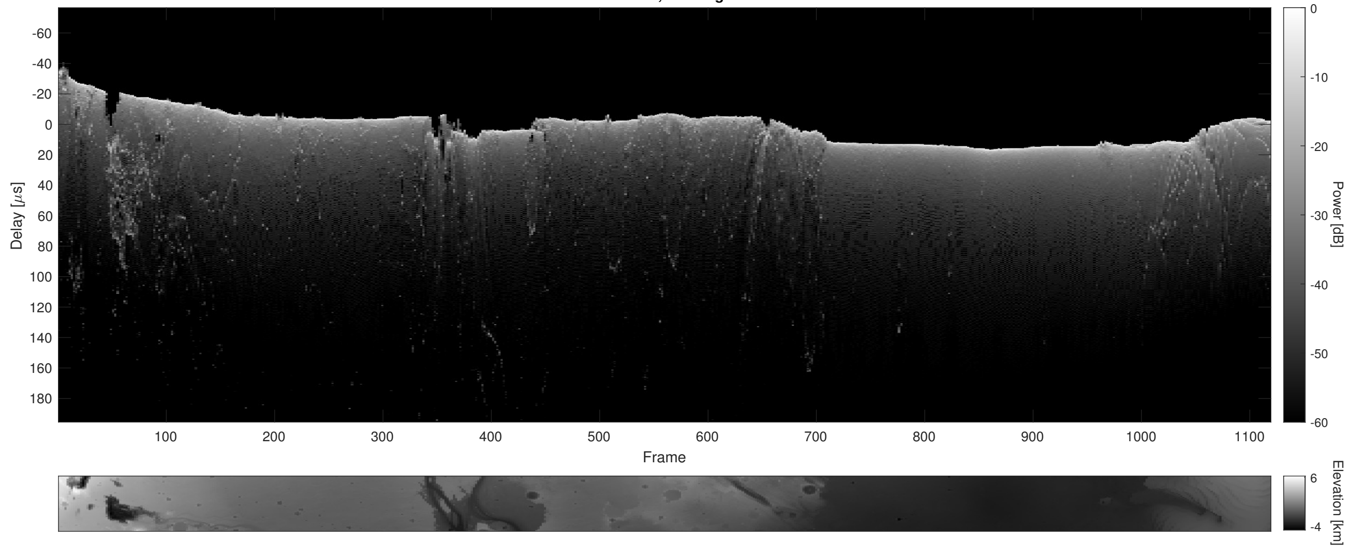
Orbit 14255, Cluttergram
