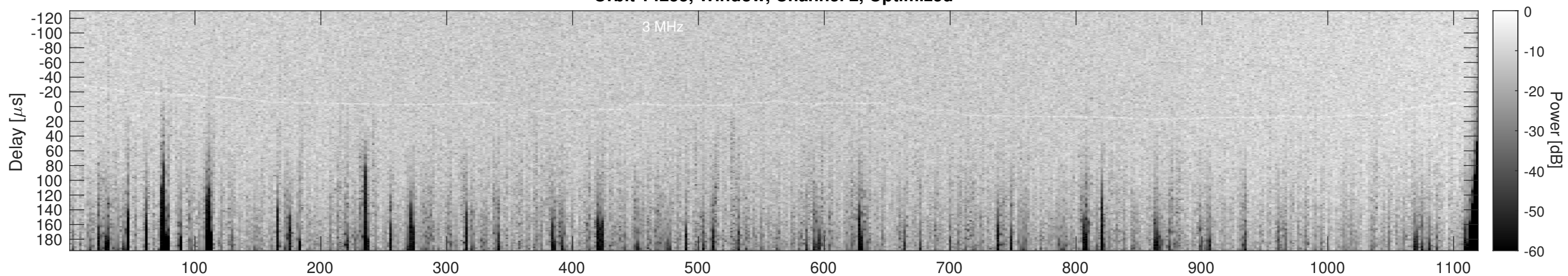
Orbit 14255, Cluttergram
