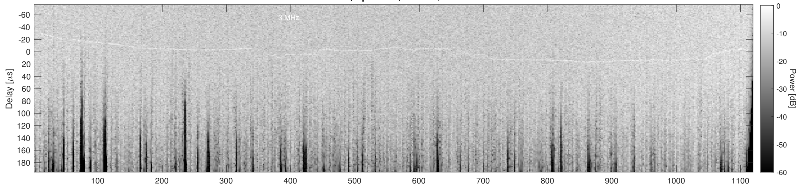
Orbit 14255, Cluttergram
