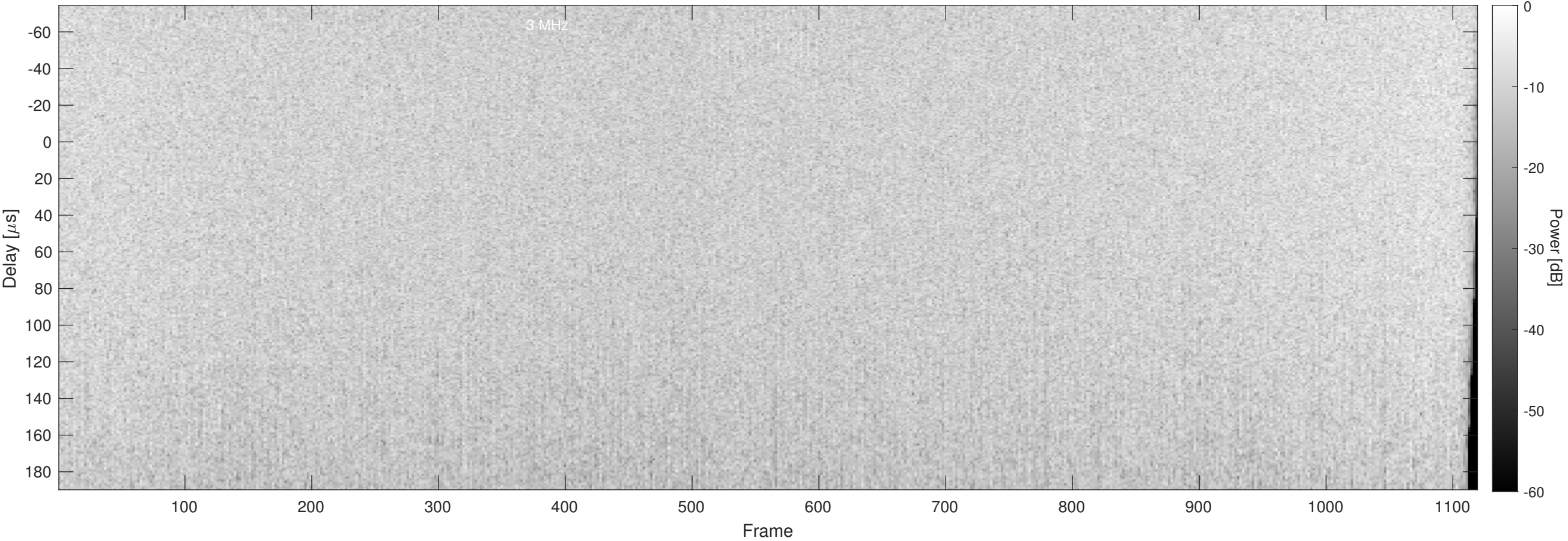
Orbit 14257, Chapman, No Window, Channel 2
