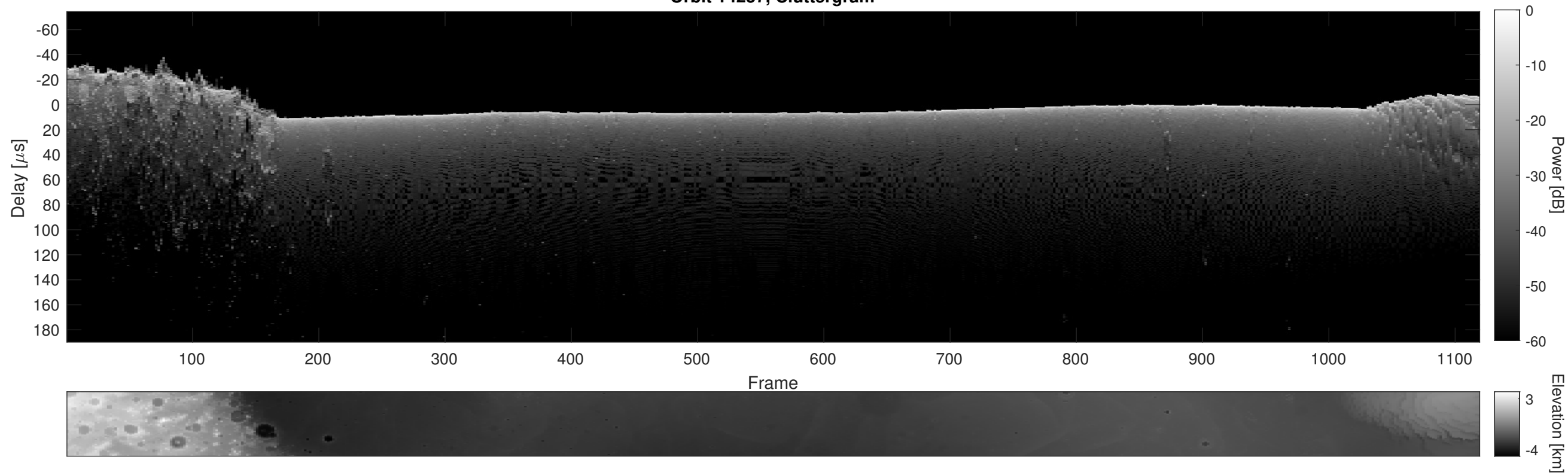
Orbit 14257, Cluttergram
