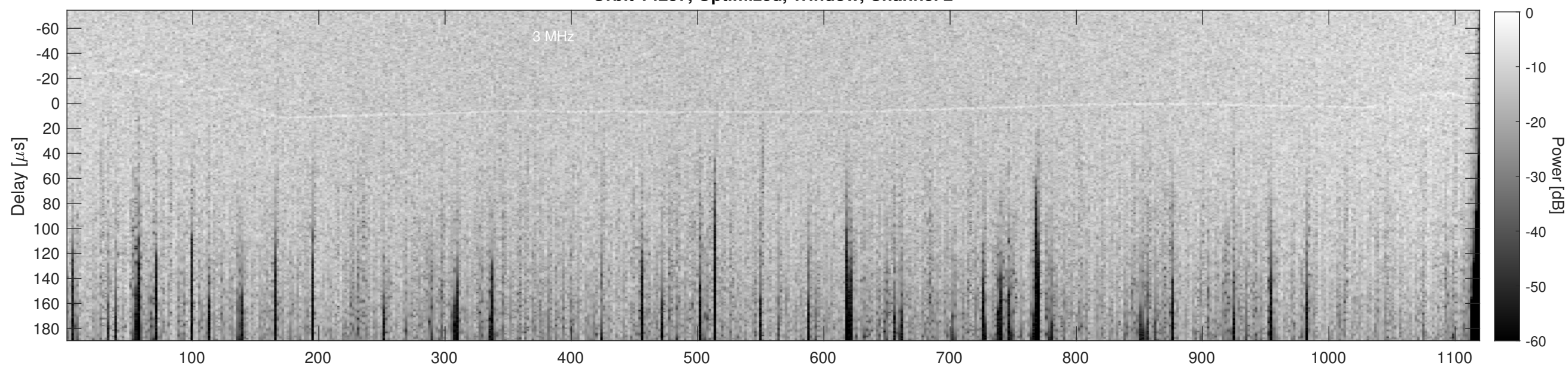
Orbit 14257, Cluttergram
