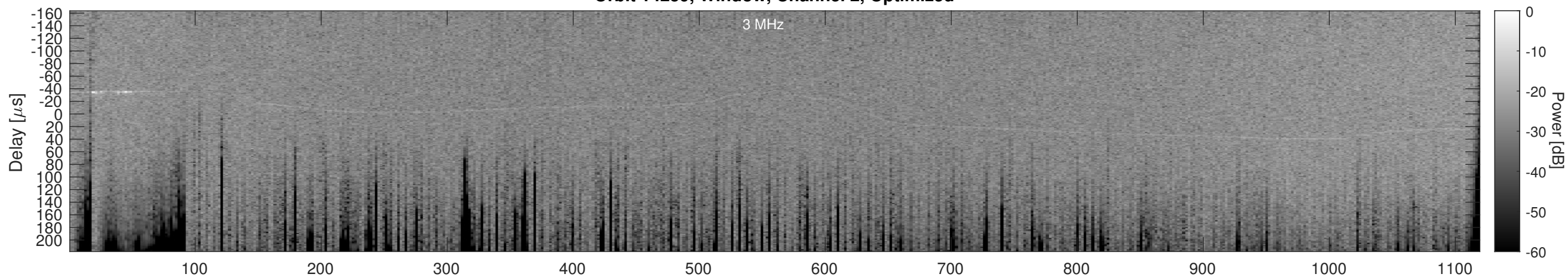
Orbit 14259, Cluttergram
