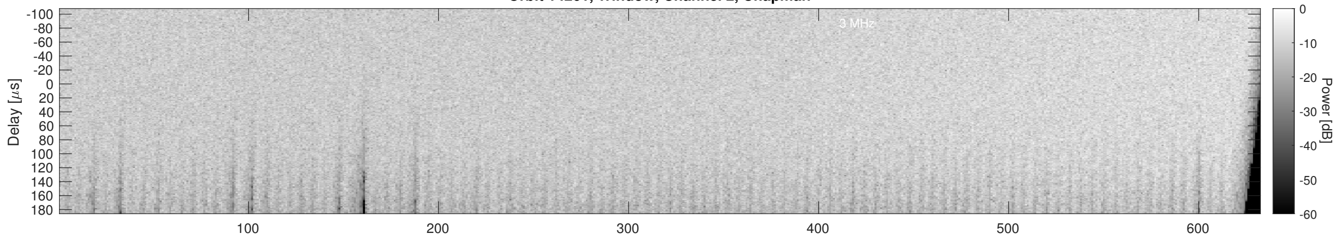
Orbit 14261, Window, Channel 2, Optimized
