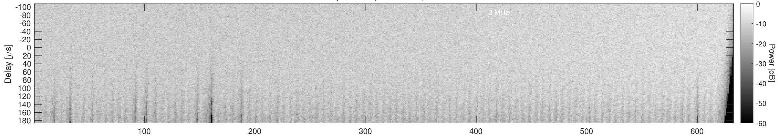
Orbit 14261, Window, Channel 2, Chapman
