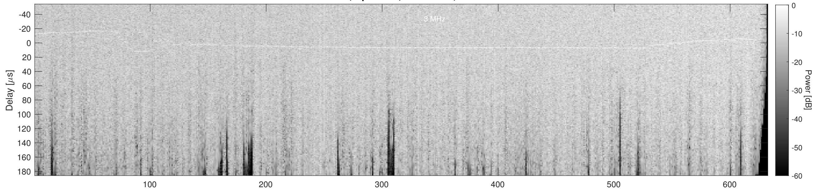
Orbit 14261, Cluttergram
