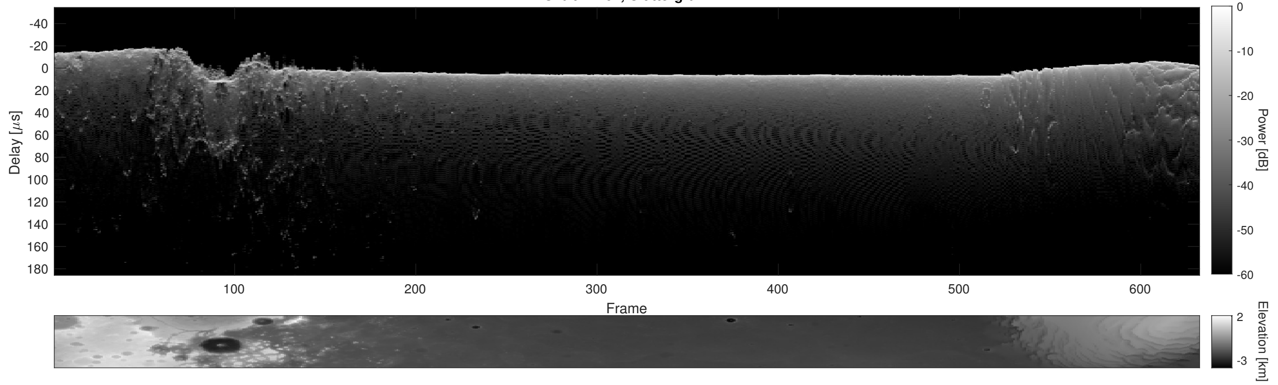
Orbit 14261, Cluttergram
