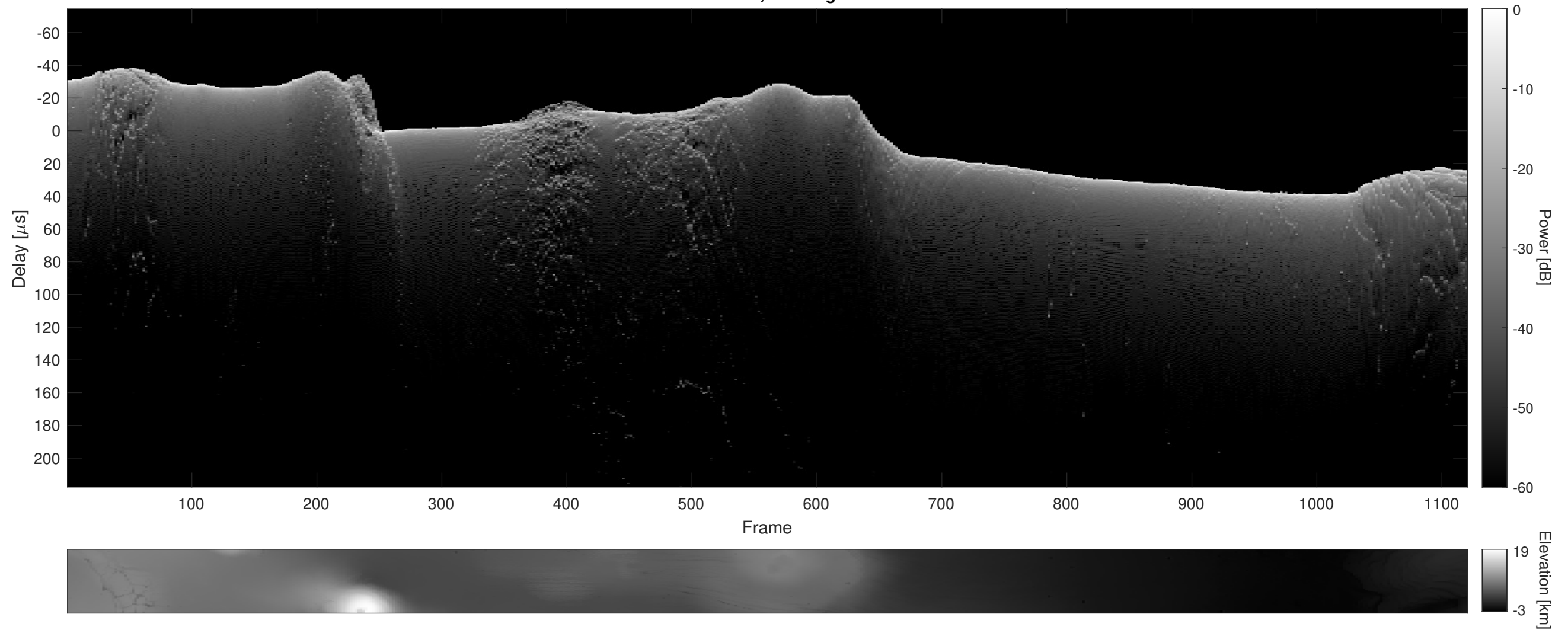
Orbit 14266, Cluttergram
